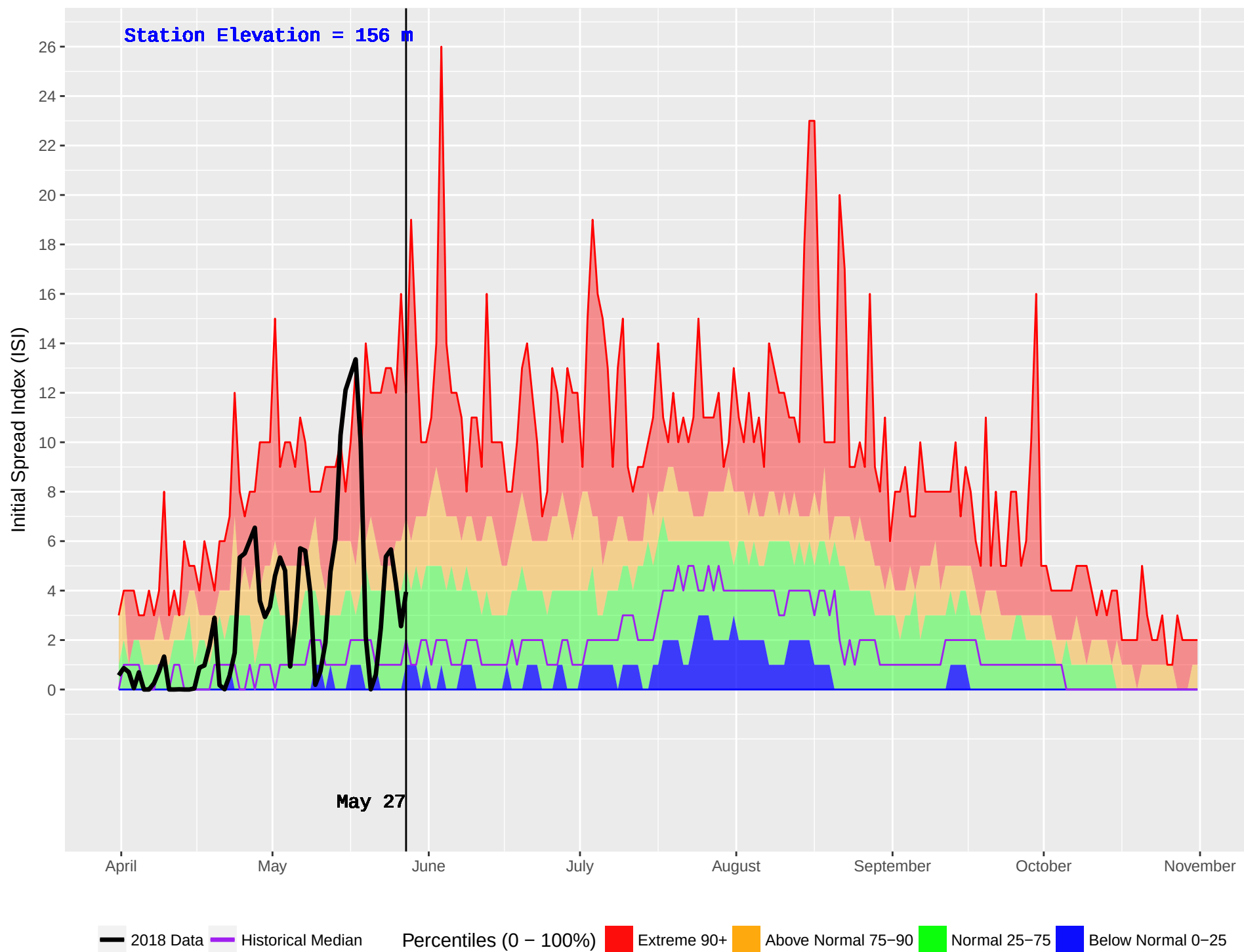
WOSS CAMP (21) : Historical (1970–2016) and Current (2018) Noon Initial Spread Index (ISI)
