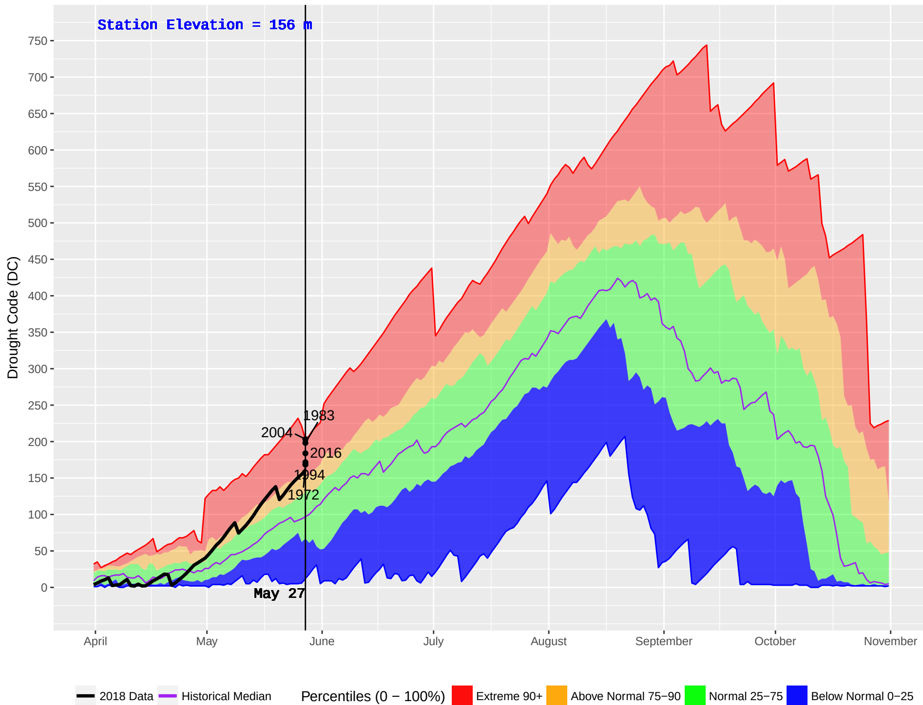
WOSS CAMP (21) : Historical (1970–2016) and Current (2018) Noon Drought Code (DC)
